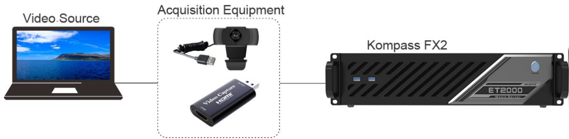
Figure 5-14 Data acquisition connection
