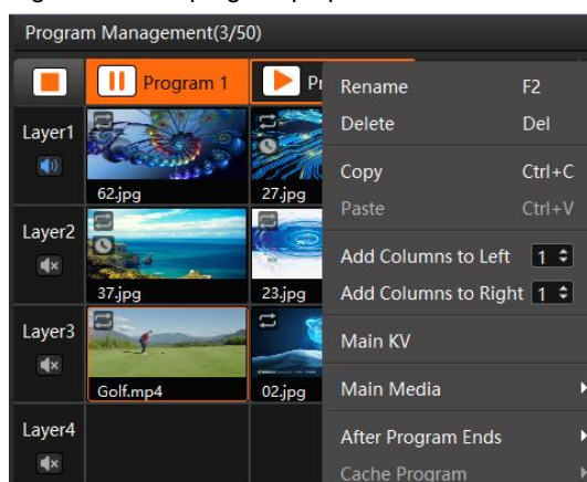
Figure 5-26 Set program properties
